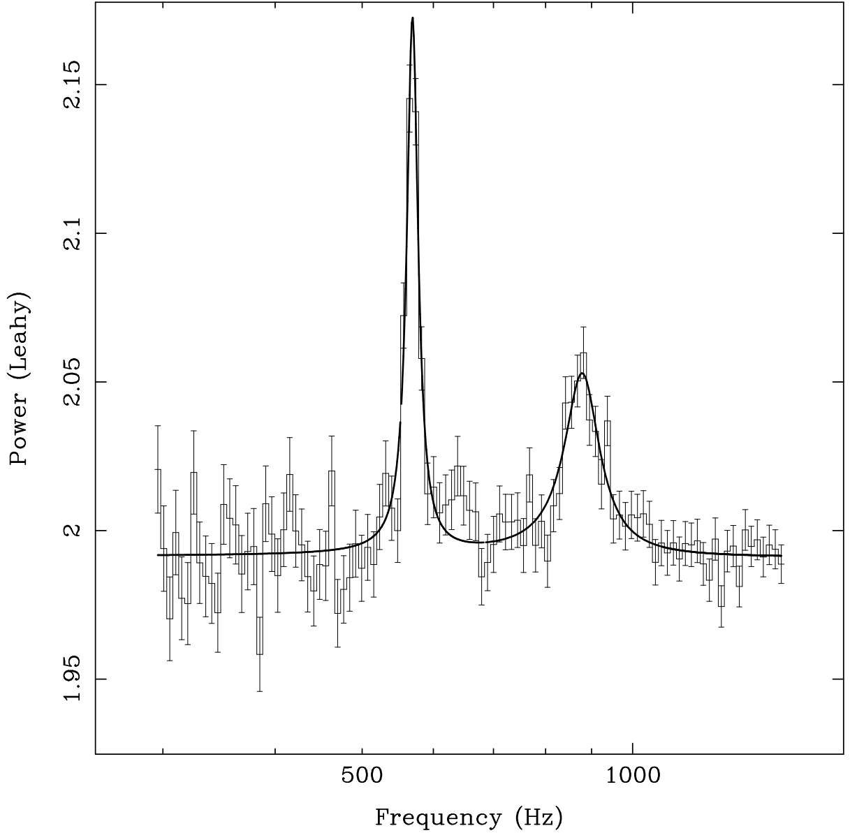
Fig. 2.— Power spectrum of a segment of 4224 s starting on UTC 1998 March 25 16:16, for the full energy band of the PCA. Both kHz QPOs are visible. No shift was applied to this power spectrum (see text). On 64 s time scales the FWHM of the lower QPO was \sim 5 Hz, but due to the variation of its central frequency during the observation it appears broader in the average power spectrum. The upper QPO was broader, and its FWHM on each segment of 64 s was \sim 100 Hz.
